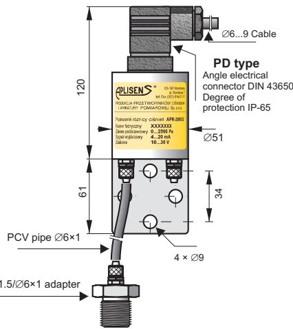
APRE-2000G Economic Version, process connection with terminal connecting to \varnothing 6 pipe ( PCV type ). An example with PD type Electrical Connection
